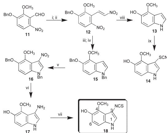
Scheme 3 Synthesis of rapalexin B ( 18 ) and thiocyanate 14 . Reagents and conditions: i, \text{CH}_3\text{NO}_2 , 18-crown-6, KF, 4-methylmorpholine, r.t.; ii, NaOAc, \text{Ac}_2\text{O} , 60 °C, 88% over two steps; iii, Fe, \text{SiO}_2 , toluene-AcOH, 90 °C, 75%; iv, NaH, THF, \text{PhCH}_2\text{Br} , 93%; v, \text{AgNO}_3 , benzoyl chloride, \text{CH}_3\text{CN} , 20%; vi, Pd/C, AcOH, \text{H}_2 /40 psi; vii, \text{CH}_2\text{Cl}_2 , \text{CaCO}_3 , \text{CSCl}_2 , 30% over two steps; viii, Pd/C, \text{H}_2 , MeOH, AcOH, 29%; ix, \text{NH}_4\text{SCN} , \text{I}_2 , MeOH, 0 °C, 49%.
